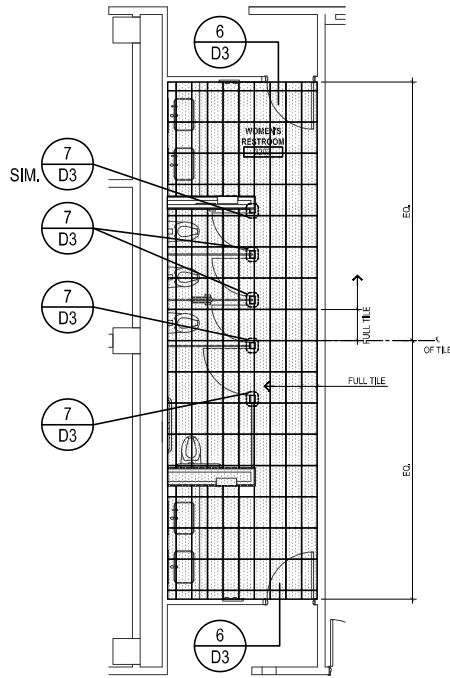
2 WOMEN'S RESTROOM 3203 SCALE: 1/8" = 1'-0" ARCH REF. : 2/A08.01
