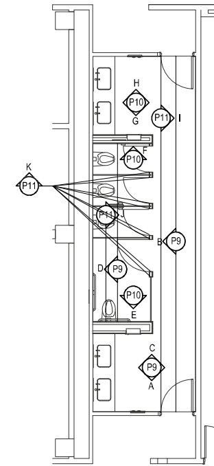
4 WOMEN'S RESTROOM 3203 SCALE: 1/8" = 1'-0" ARCH REF. : 2/A08.01
