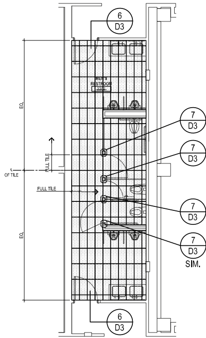
1 MEN'S RESTROOM 3202 SCALE: 1/8" = 1'-0" ARCH REF. : 1/A08.01
