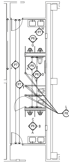
3 MEN'S RESTROOM 3202 SCALE: 1/8" = 1'-0" ARCH REF. : 1/A08.01
